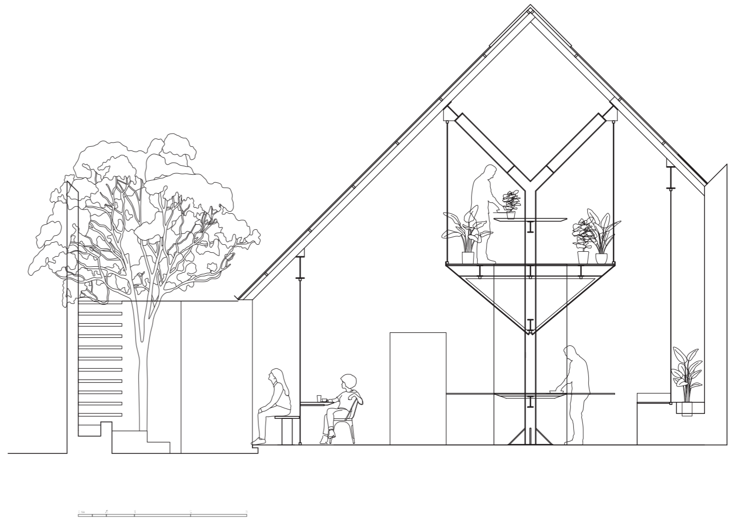
SECTION
